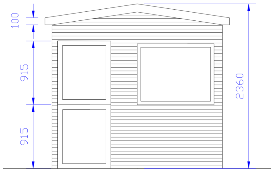
Figure 1 – Standard Beach Hut Front Elevation Option
